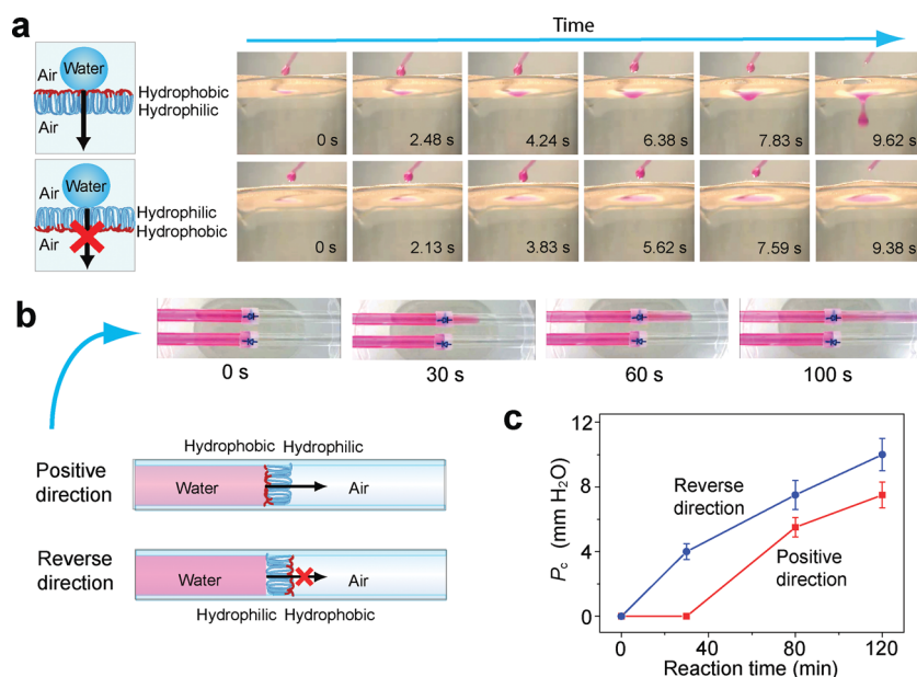
Figure 2. Directional water droplet and flow penetration across Janus-C in air-water systems. a) Unidirectional droplet penetration demonstrated by dropwise addition of water droplets ( \approx 20 \mu\text{L} per droplet, dyed red with rhodamine 101) onto hydrophobic side (top) and hydrophilic side (bottom) of Janus-C. b) Schematics and sequential snapshots showing unidirectional water flow penetration through Janus-C. The membrane was sandwiched between two glass tubes (tube volume of \approx 10 mL and inner diameter \approx 1 cm), and water (3.5 mL) was loaded respectively on the hydrophobic (upper) and hydrophilic sides (lower) of Janus-C. c) Anisotropic critical breakthrough pressure ( P_c ) of Janus membranes prepared with different reaction time.
