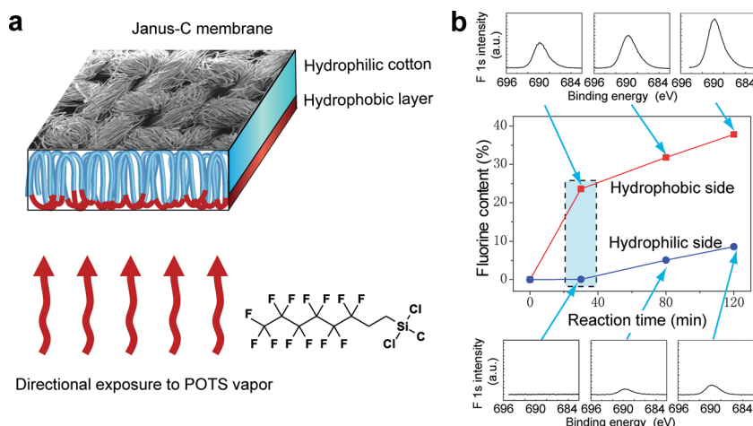
Figure 1. Preparation of Janus-C. a) Schematic illustration of the preparation method where vapor of POTS diffuses towards a cotton membrane and reacts with its surface hydroxyl groups, creating a through-plane chemical gradient. Careful control of reaction conditions renders the exposed side hydrophobic and the other side hydrophilic. b) XPS analysis of F 1s peaks on both sides of the Janus membranes with different reaction time. The green rectangle indicates Janus-C.
