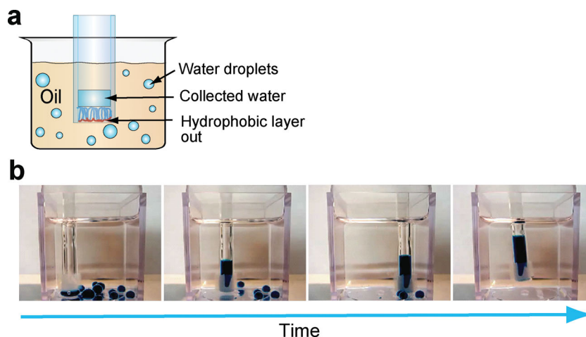
Figure 4. Water droplet scavenging using Janus-C. (a) Scheme showing the construction of “Janus trapper” for water droplet collection from oil. (b) Sequential snapshots showing effective collection of water droplets (dyed blue by methylene green) from oil (hexadecane) by the Janus trapper.
