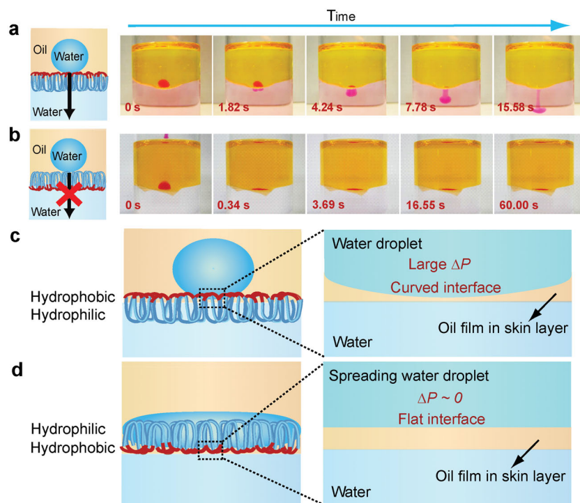
Figure 3. Directional water droplet penetration across Janus-C in oil-water systems. a) Janus-C allows penetration of water droplet (dye red) when the hydrophobic side is towards oil (hexadecane dyed yellow by Nile red), b) and prevents droplet penetration when reversely aligned. c) For positively aligned Janus-C, a water droplet touching the hydrophobic side exerts a larger Laplace pressure ( \Delta P ), creating a larger driving force for penetration. Consequently, the water droplet can penetrate through the thin oil-infused skin layer and further across the whole membrane. d) For reversely aligned Janus-C, a water droplet touching the hydrophilic side tends to spread, exerting limited Laplace pressure. The oil-infused skin layer is thus able to block its penetration.
